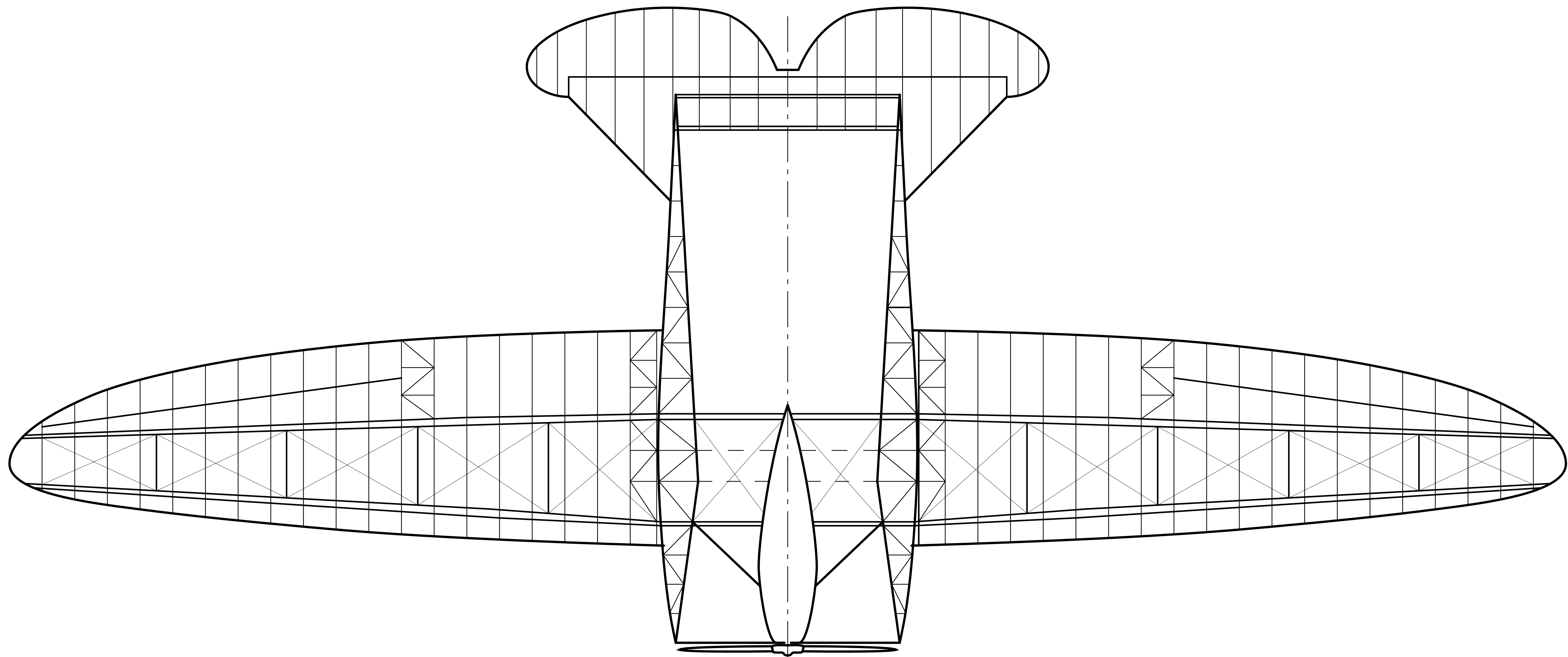
Stipa - Caproni Scale 1/20
